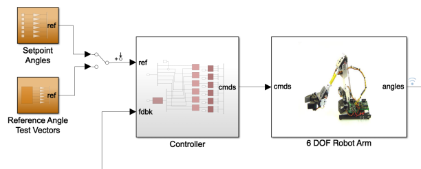
Fig. 2 A Simulink model of the electrical and mechanical components of the robotic arm. Reproduced with permission of MathWorks. Copyright (2020) [1]
