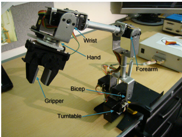
Fig. 1 Six degree-of-freedom robotic arm. Reproduced with permission of MathWorks. Copyright (2020) [1]
