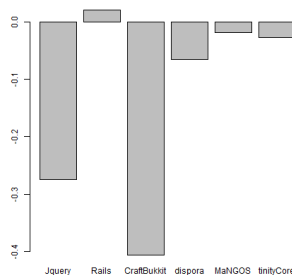
Fig. 2: Emotion score average per project, using SENTISTRENGTH (replication).
