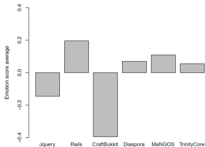
Fig. 1: Emotion score average per project, using SENTISTRENGTH [33].
