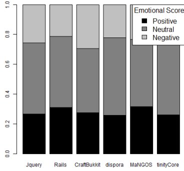
Fig. 5: Proportion of positive, neutral and negative commit comments per project, using SENTISTRENGTH (replication).
